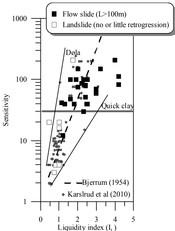
Figure 5: Liquidity index plotted against sensitivity for quick clay landslides observed in Norway.
