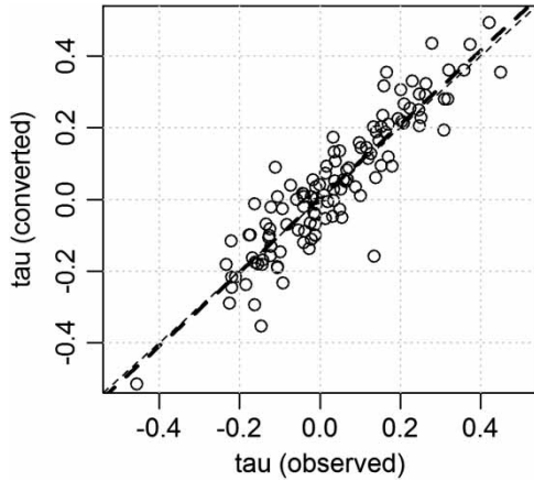
Figure 1 | Comparison of the calculated Mann-Kendall trend estimates ( \tau -values) between the observed and converted SD time series from a same set of 120 stations. The thin and thick dashed lines denote perfect fit and a linear regression fitted to the points, respectively.
