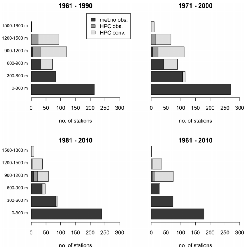
Figure 2 | Distribution of stations in different elevation intervals and time periods. The darkest shading denotes analyzed time series from met.no station network, and the lighter shadings observed and converted time series from the stations of the hydropower companies (HPC).
