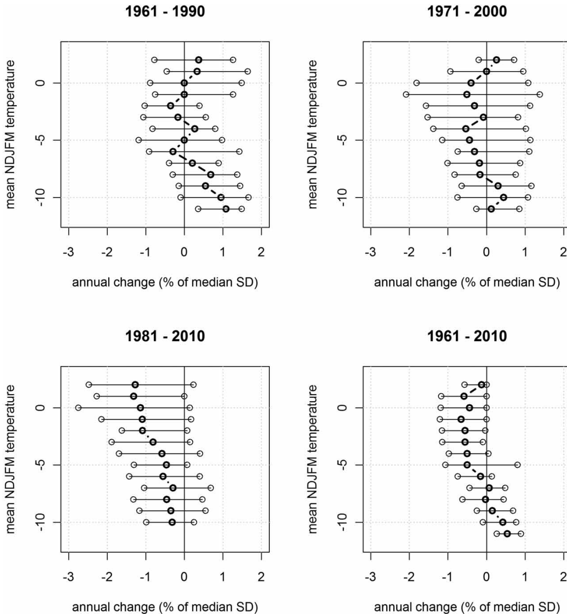
Figure 7 | The distribution of the relative annual trend slope magnitudes in SD in the four periods, binned by mean winter (NDJFM) temperature of the period. The thick circles in the middle denote the medians of the distributions per temperature bin, and the error bars the 10 and 90% percentile intervals. Only those temperature bins with time series from more than 15 stations are included.
