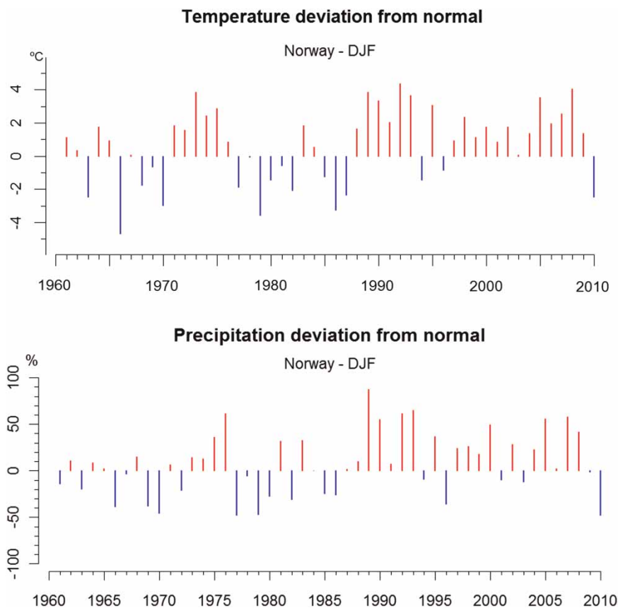
Figure 4 | The deviations of winter (DJF) temperature (upper) and precipitation (lower) from 1961–1990 normal period means.
