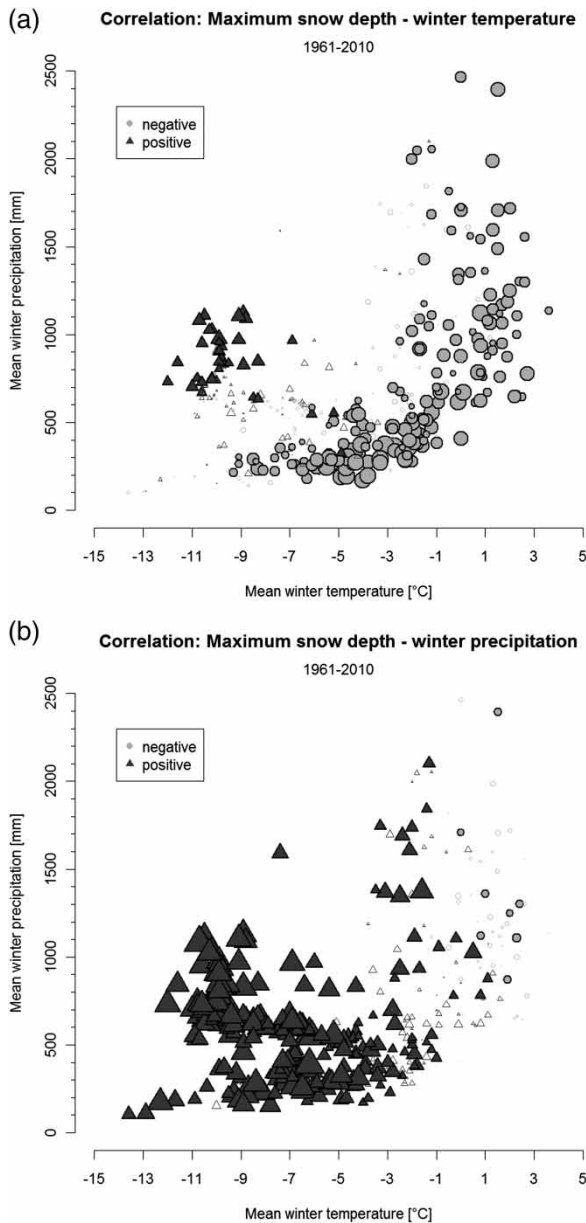
Figure 8 | Correlation between annual maximum SD in 1961–2010 and (a) winter (NDJFM) temperature and (b) winter precipitation, plotted against mean winter climate. Circles denote negative correlation, and triangles positive correlation. The larger the symbol the stronger the correlation (the legend symbol size indicate a Kendall's tau coefficient of 0.5). Outlined symbols denote correlations that are statistically significant (i.e. significantly different from zero) at the 0.05 alpha level.
