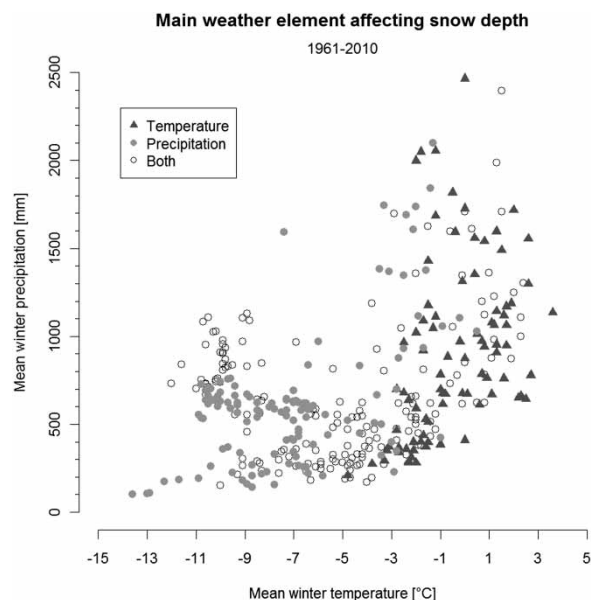
Figure 10 | Stations with clearly temperature dominated (triangle) precipitation dominated (circle) maximum snow depth regime. Open circles denote stations where neither temperature nor precipitation alone dominates variations in SD.
