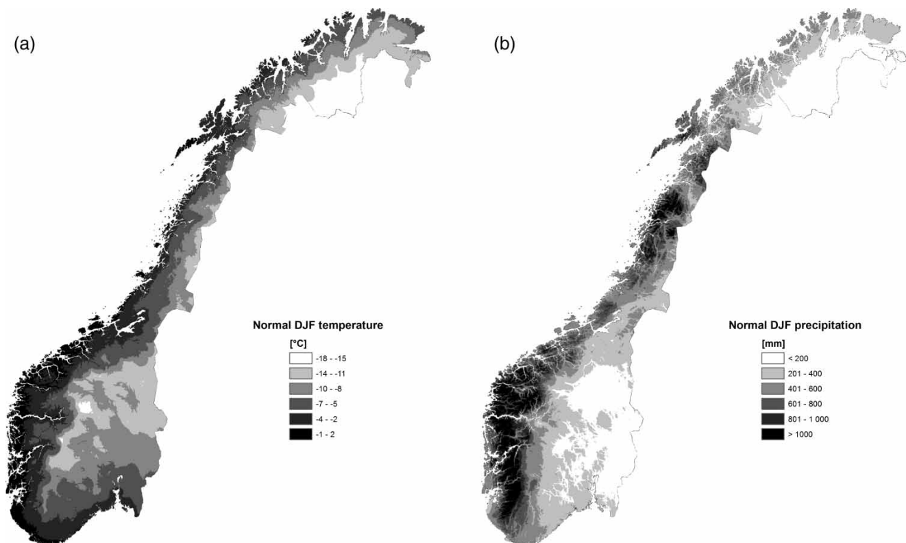
Figure 3 | Average winter (DJF) temperature (left) and precipitation (right) for the standard normal period 1961–1990.
