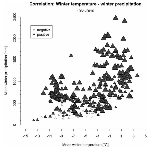
Figure 9 | Correlation between winter temperature and winter precipitation, plotted against mean winter climate. Circles denote negative correlation, and triangles positive correlation. The bigger the symbol the stronger the correlation, and outlined symbols denote correlations that are statistically significant (i.e. significantly different from zero) at the 0.05 alpha level.
