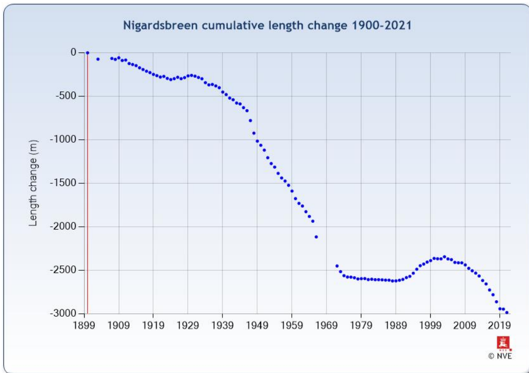
Figure 3. Example of a length change product from Nigardsbreen.
