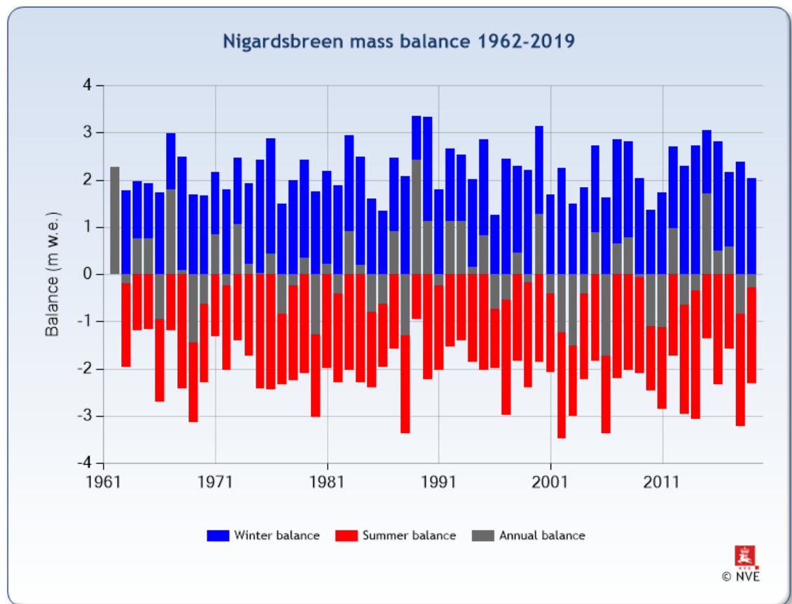
Figure 2. Example of a mass balance product from Nigardsbreen.
